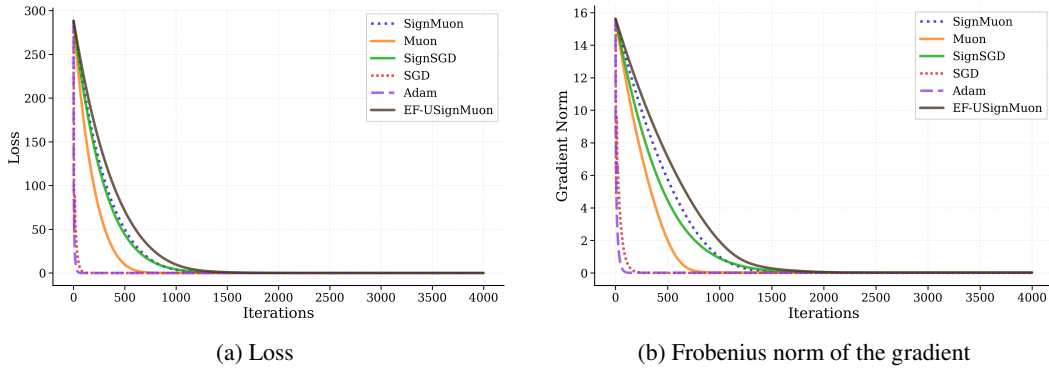
Figure 3: Smooth convex problem (Equation 12 for 500 \times 500 ).
