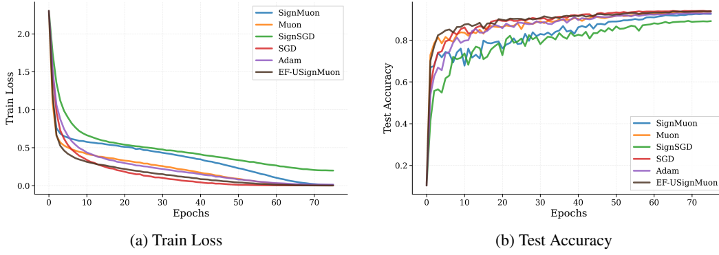
Figure 2: Centralized setting. Comparison of convergence and classification accuracy achieved by different optimization algorithms while training a ResNet-18 classifier on CIFAR-10.
